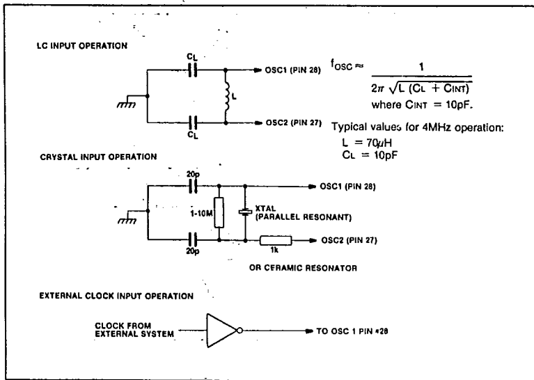
Fig.10 Oscillator options
