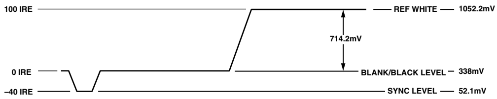
Figure 113. NTSC Luma Video Levels
