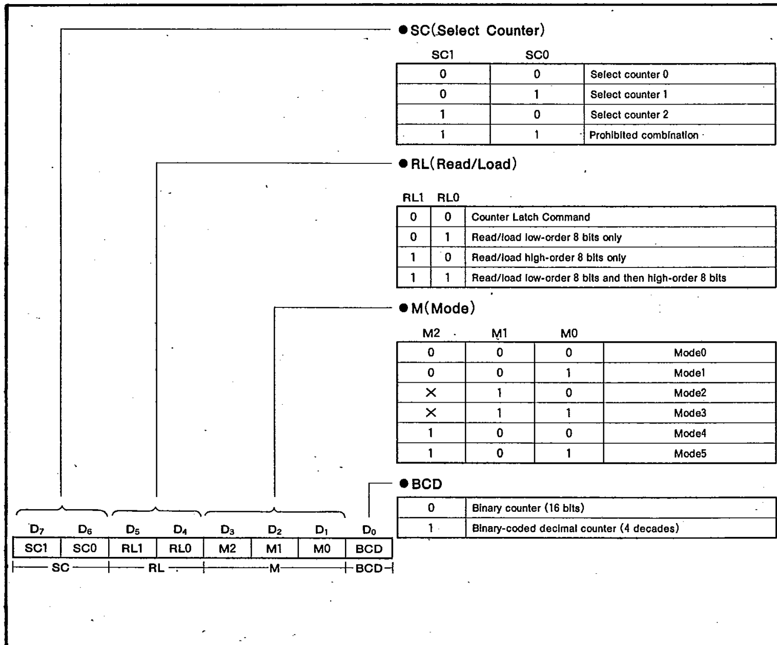
Fig. 1 Control-Word Format
