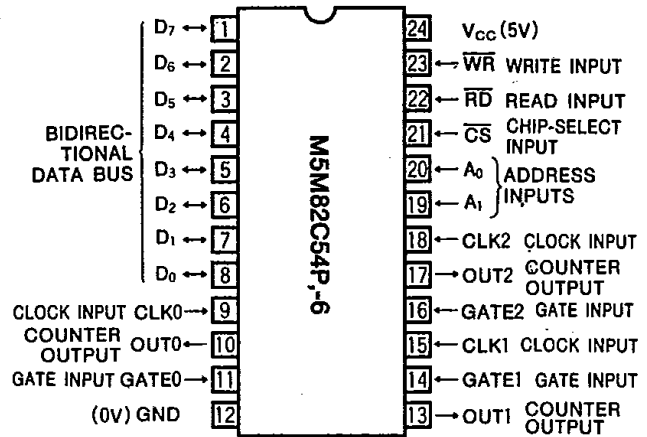
Outline 24P4
