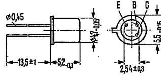
Approx. weight 0.33 g Dimensions in mm
