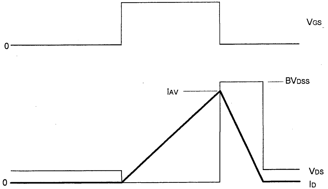
Fig.2 Operating waveforms
