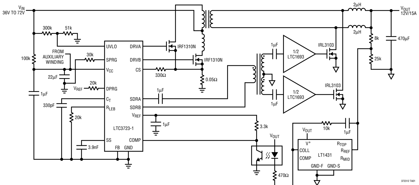
Isolated 36V to 72V DC to 12V/15A Push-Pull Converter
