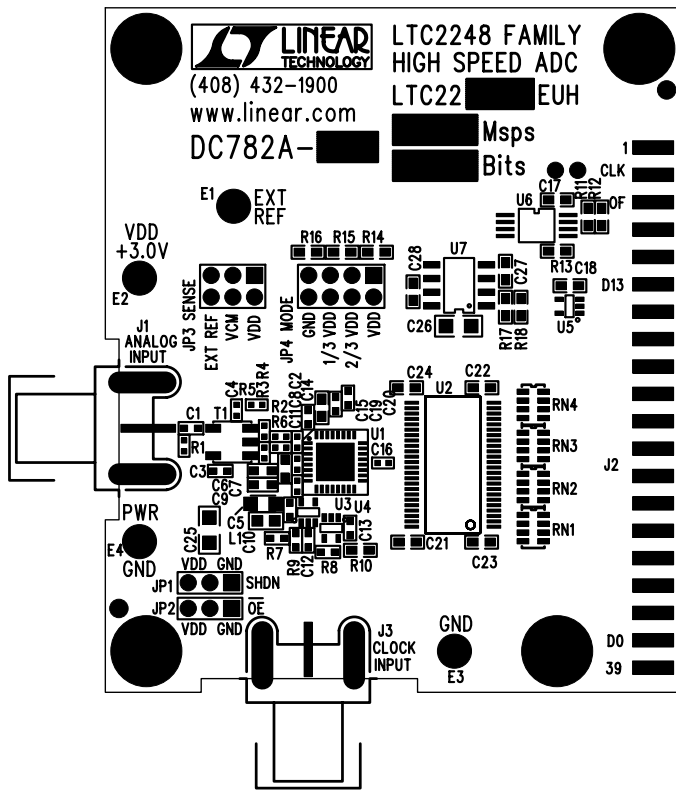
Silkscreen Top
