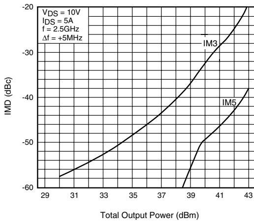
IMD vs. OUTPUT POWER
