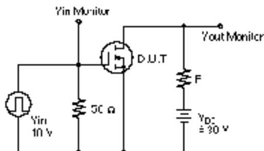
Sv Timing Time Test Circuit
