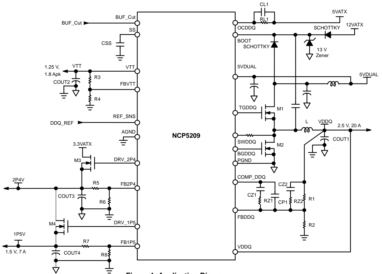
Figure 1. Application Diagram
