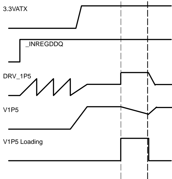
Figure 3. Hiccup Mode Soft-start of Dual Linear Regulators
