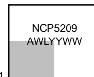
20-LEAD QFN MN SUFFIX CASE 505
