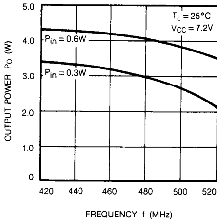
OUTPUT POWER VS. FREQUENCY
