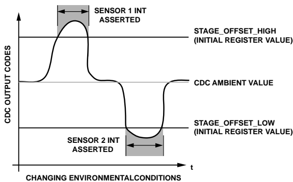
Figure 23. Ideal Sensor Behavior with a Constant Ambient Level
