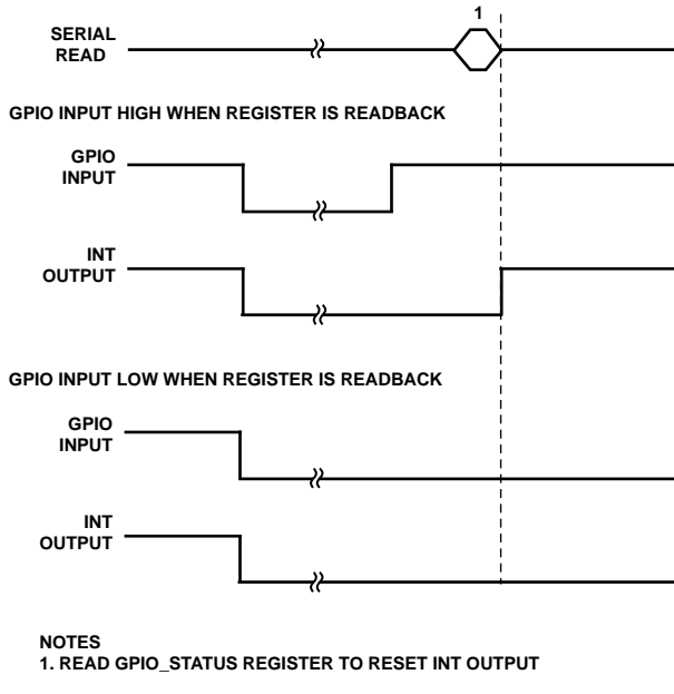
Figure 29. \overline{INT} Output Controlled by the GPIO Input Example, GPIO\_SETUP = 01 , GPIO\_INPUT\_CONFIG = 00
