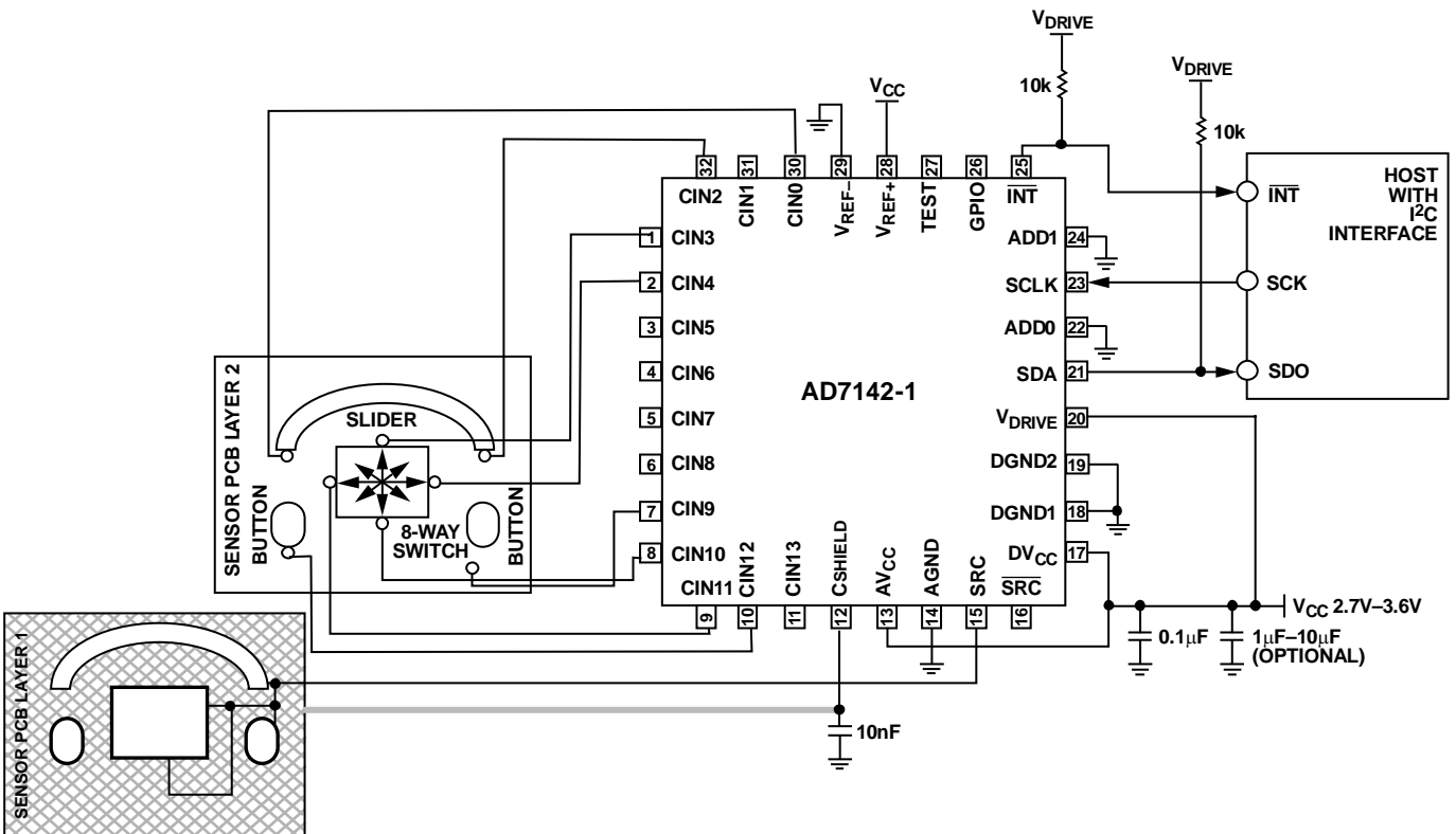
Figure 46. Typical Application Circuit with I 2 C Interface
