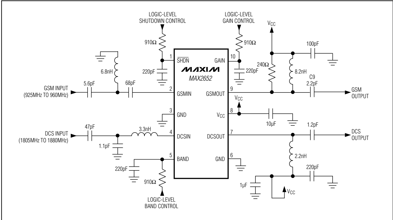
Figure 2. MAX2652 Typical Application Circuit
