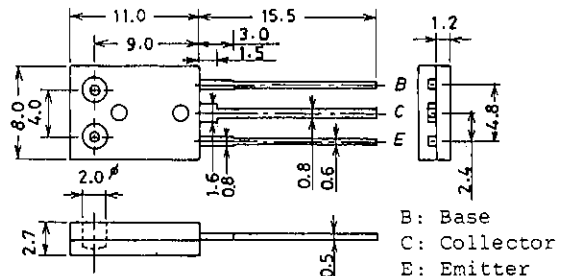
Package Dimensions 2043A (unit:mm)
